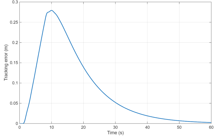
Fig. 3. Position tracking error between bicycle and cargo cart.
