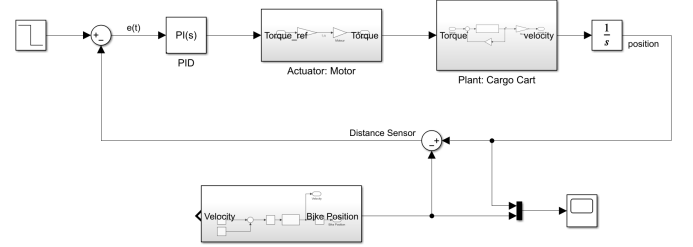
Fig. 1. Closed-loop model of the bicycle-cargo system with PI control.
