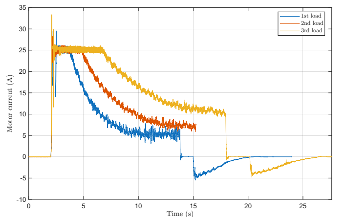
Fig. 4. Measured motor current under three loading conditions.
