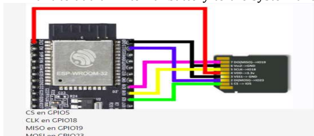
Figure 7: ESP32 connection with SD card
