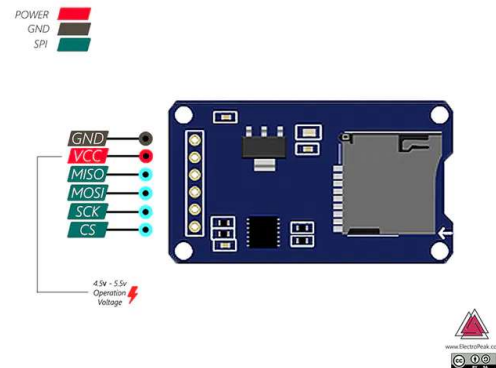
Figure 6: Micro SD-adapter for Arduino boards
